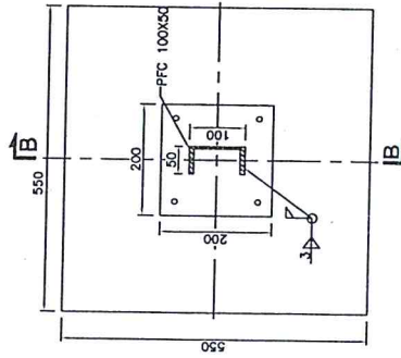
CONCRETE BLOCK DETAIL
